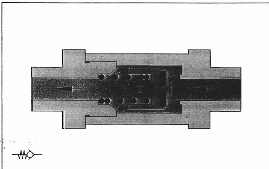
Check valve
