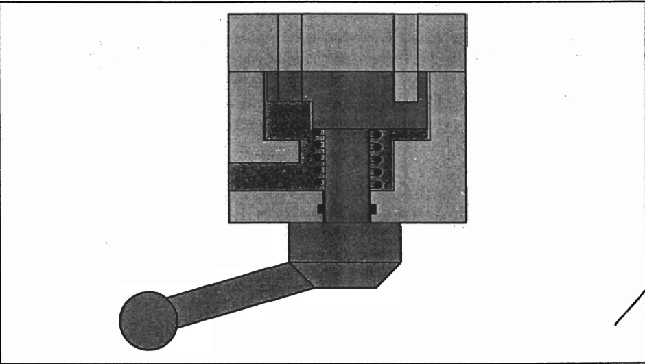
4/3 way plate slide valve, cross section
