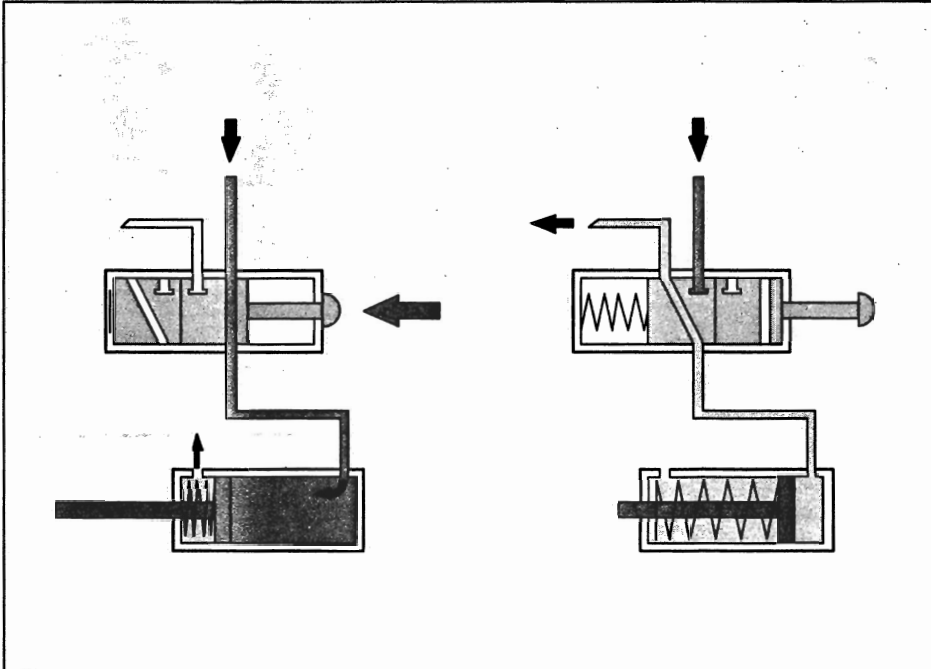
Control of a single acting cylinder
