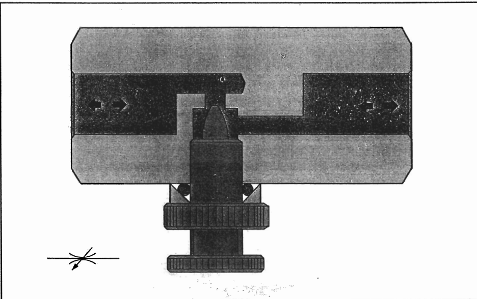
Throttle valve
