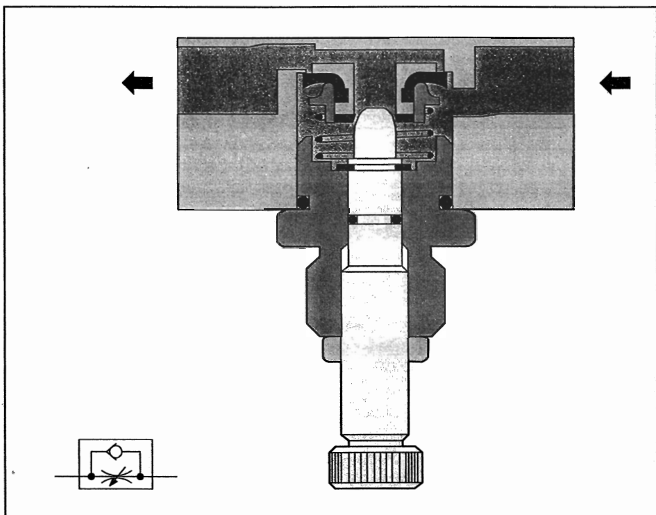
One way flow control valve
