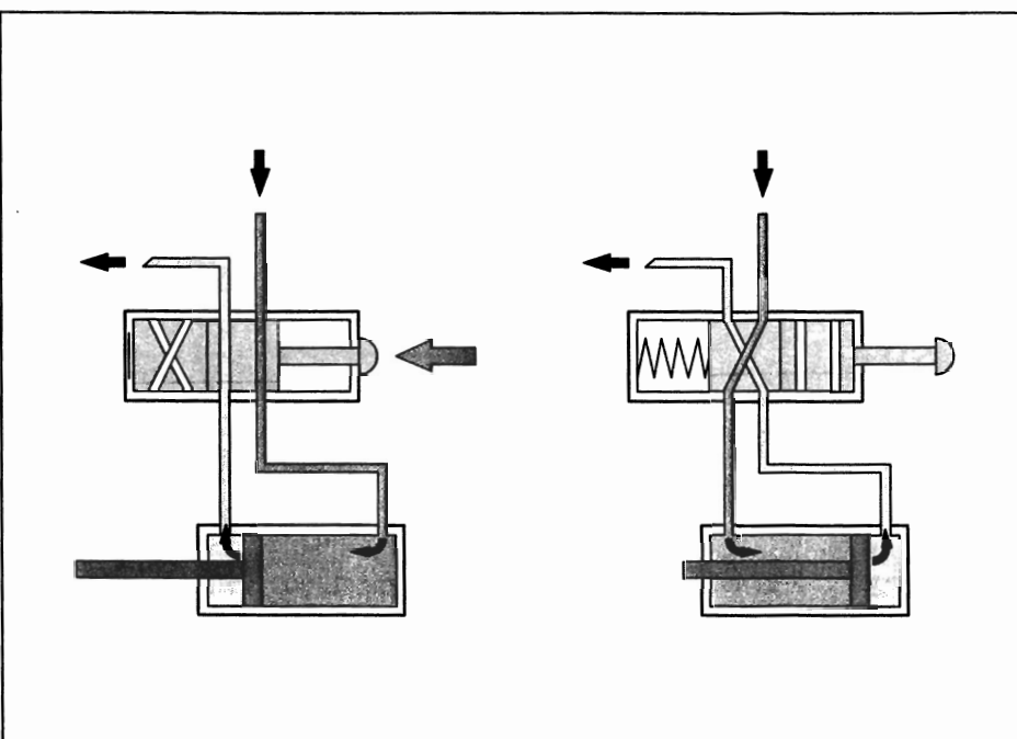
Control of a double acting cylinder
