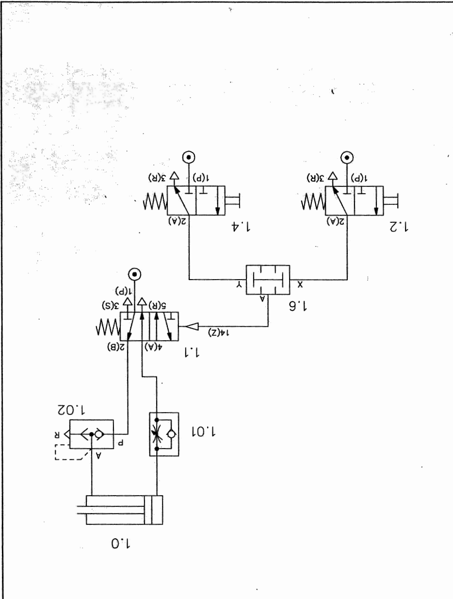
Circuit diagram
