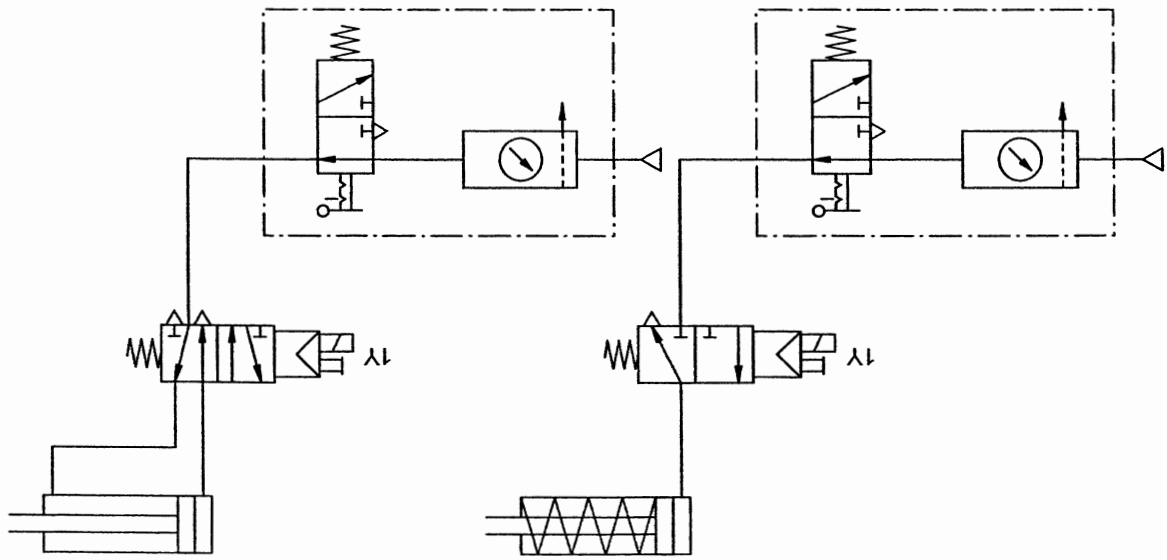
Fig. 5/2: Circuit diagram, pneumatic
