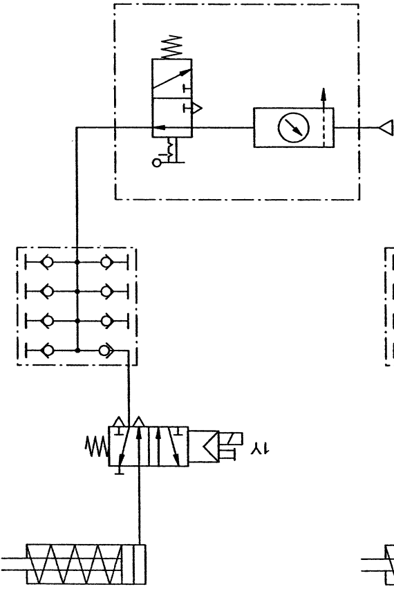
Fig. 1/2: Circuit diagram, pneumatic
