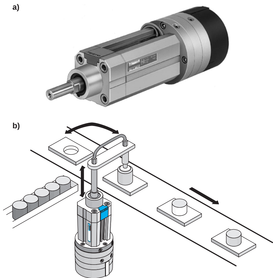
Fig. 9.3: Rotary/linear drive (Festo)
