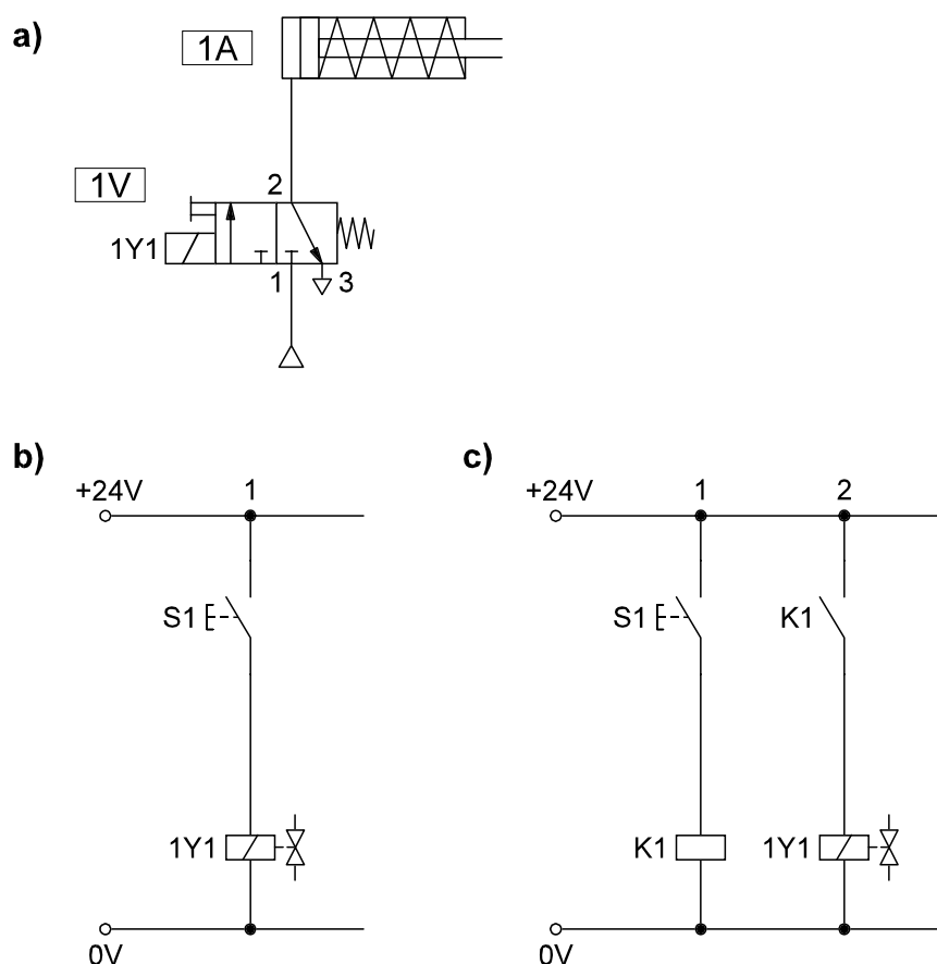
Fig. 8.1: Circuit diagrams for control of a single-acting cylinder
