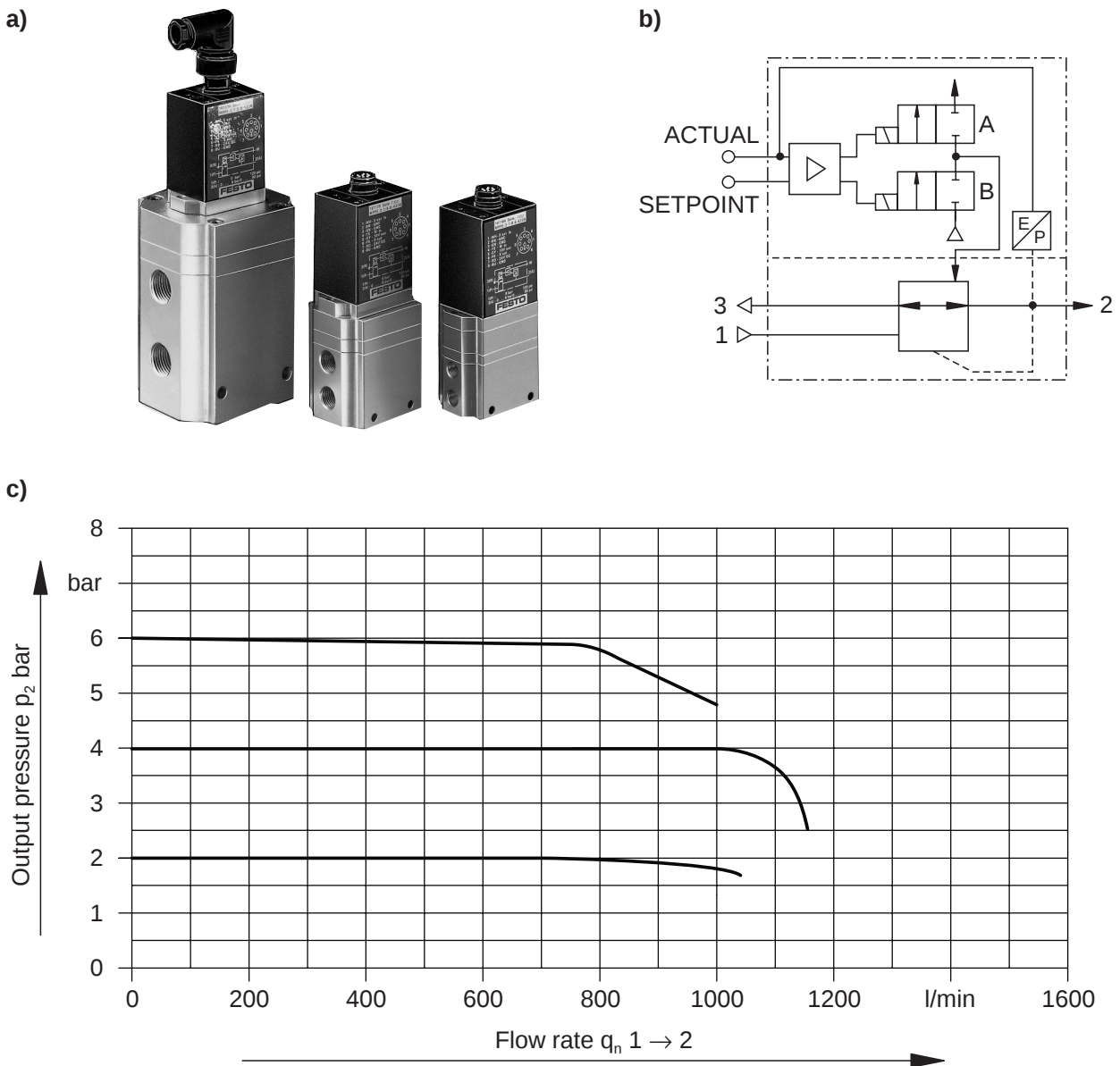
Fig. 9.18: a) Valves of different nominal sizes, Proportional pressure regulating valves b) Equivalent circuit diagram, c) Pressure/flow rate characteristics
