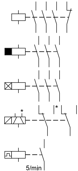
Fig. 6.26: Graphical symbols for relays and contactors (consolidated representation)
