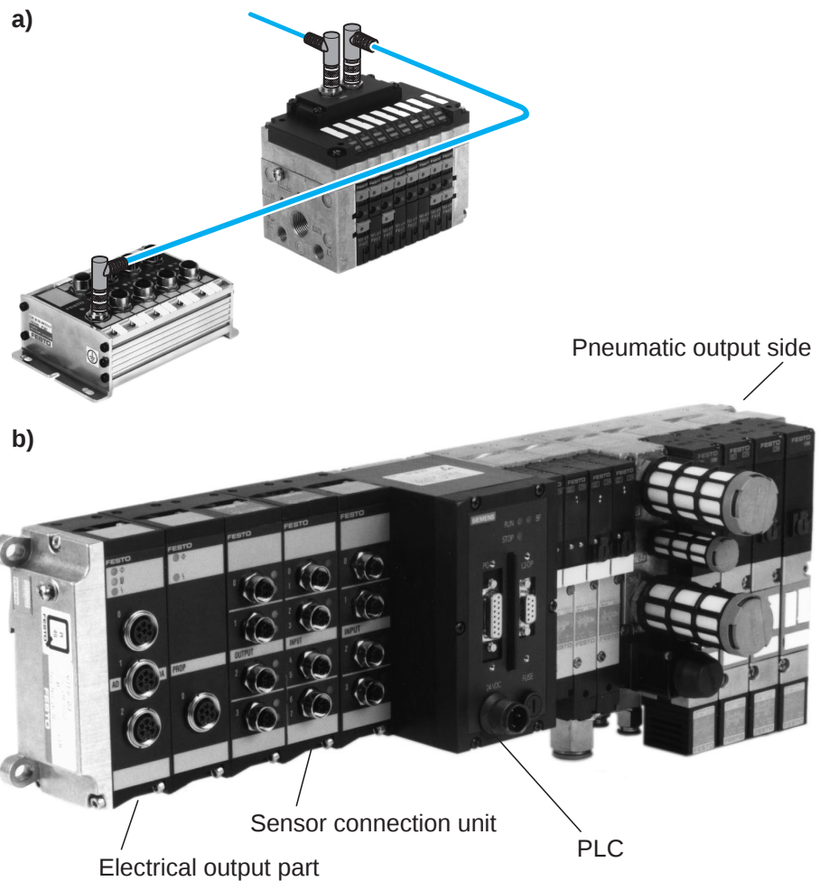
Fig. 9.9: Control components for reduced installation effort
