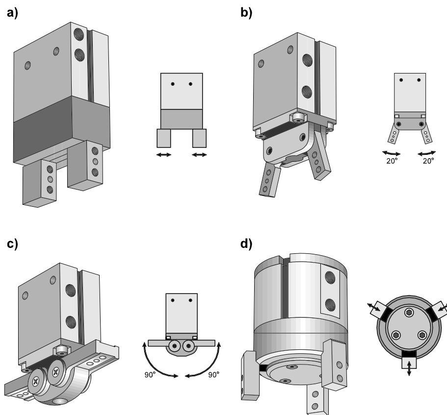
Fig. 9.4: Pneumatic grippers
