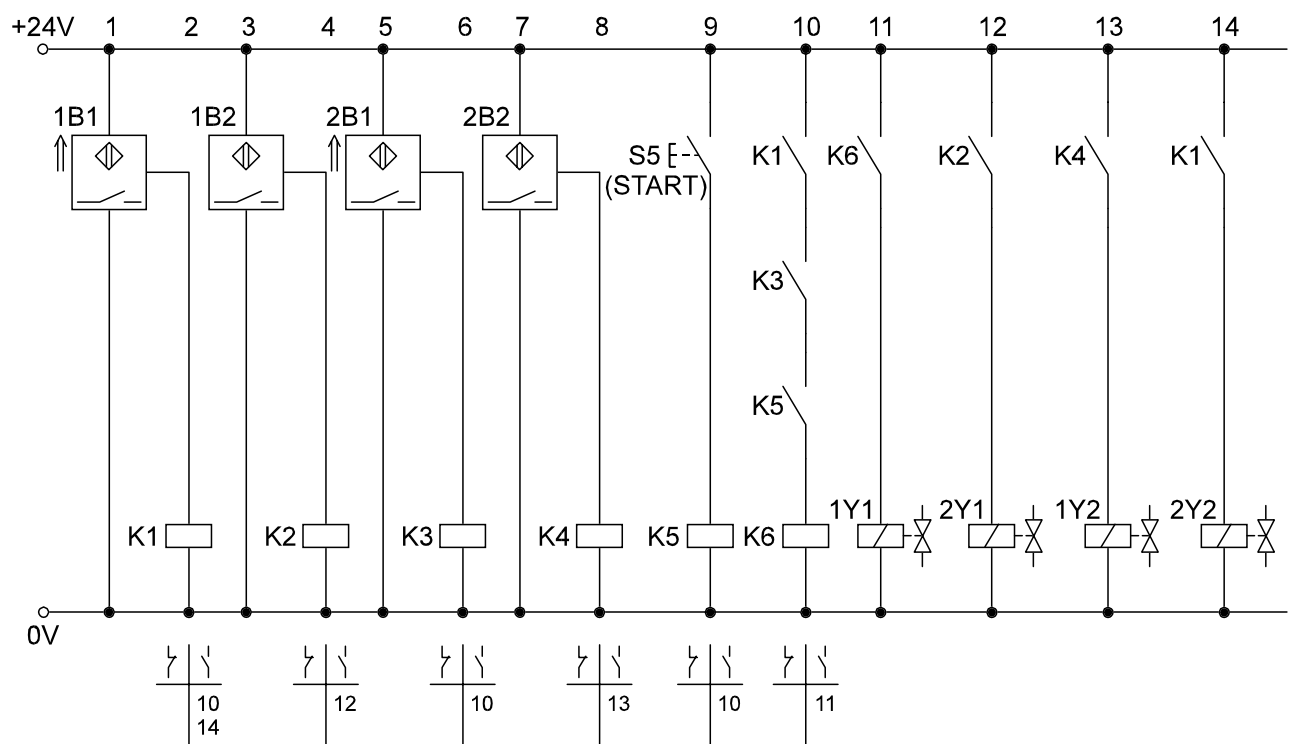
Fig. 8.19: Electrical circuit diagram of the feeding device
