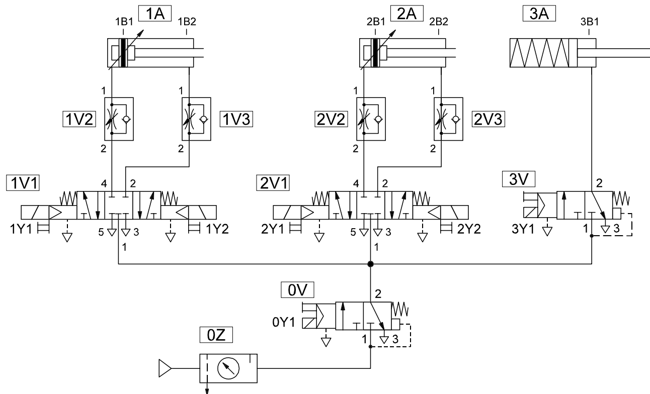
Fig. 8.24: Pneumatic circuit diagram of the lifting device
