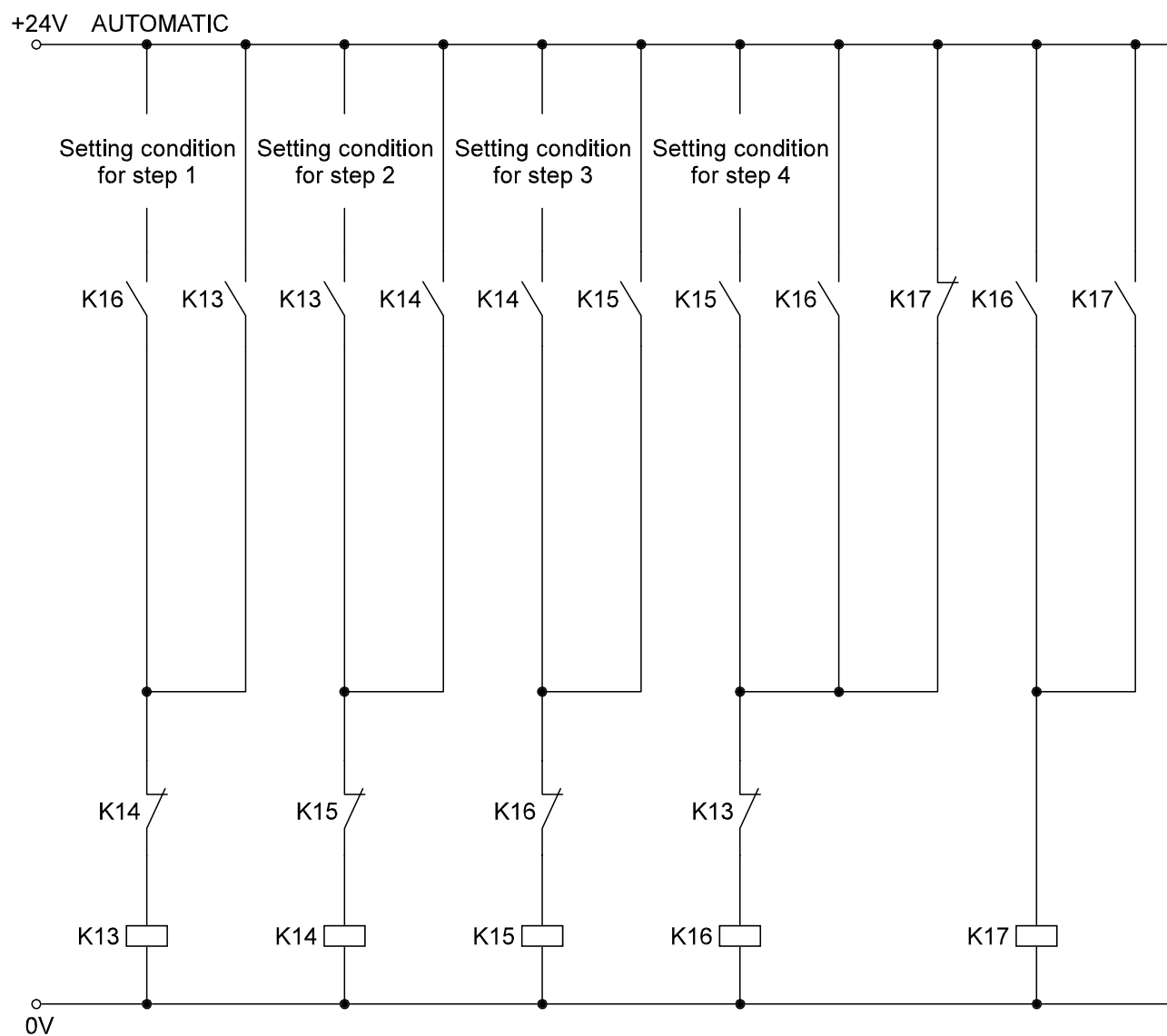
Fig. 8.28: Schematic design of a reset sequencer for the lifting device
