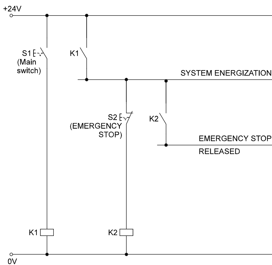
Fig. 8.22: Relay circuit for the main switch and EMERGENCY STOP control elements
