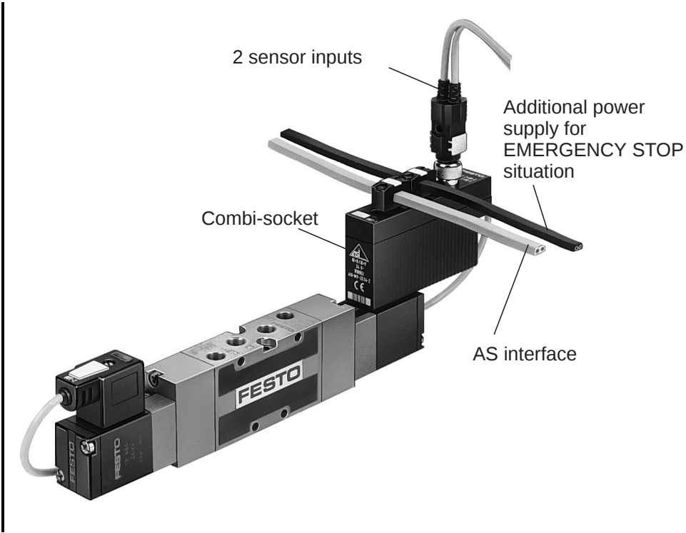
Fig. 9.11: Directional control valve with AS interface
