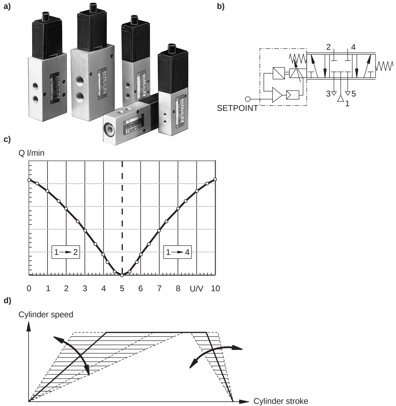
Fig. 9.19: Proportional directional control valves
