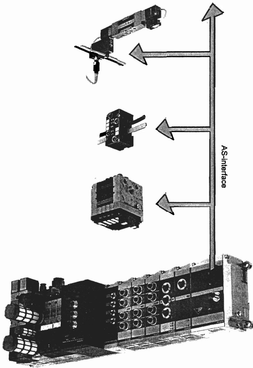
Fig. 9.16: Design of an electro- pneumatic control system using the AS-interface
