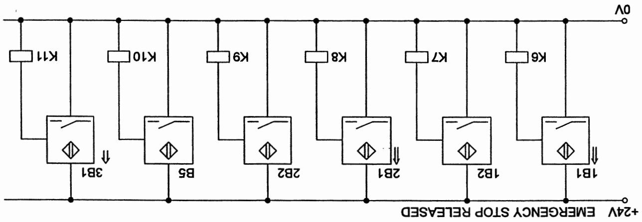
Fig. 8.25: Relay circuit diagram for sensor evaluation
