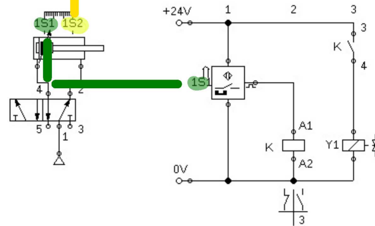
Electronneumatic
